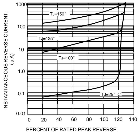
FIG.4-TYPICAL REVERSE
