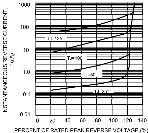
FIG.5-TYPICAL REVERSE CHARACTERISTICS
