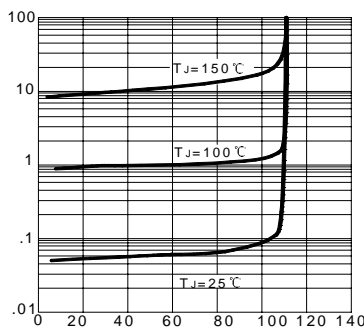
FIG.6 – TYPICAL REVERSE CHARACTERISTICS
