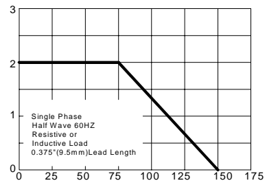
FIG.3 – FORWARD DERATING CURVE
